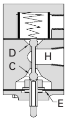
Throttling Pilot
