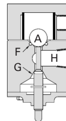
Envirosave™ Pilot
